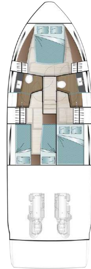
LOWER DECK
